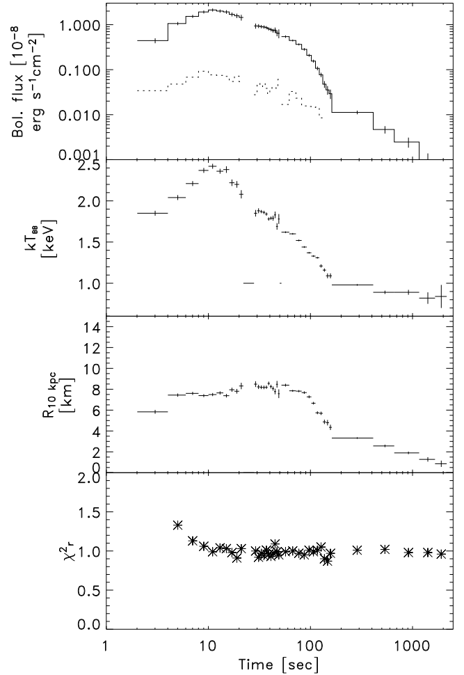
Fig. 5. Modeling results for time-resolved 0.7–10 keV burst spectra of 14 bursts detected XMM-Newton observation. Spectral channels were binned so that each bin contains at least 15 photons. The number of degrees of freedom ranges between roughly 500 and 2000 (for 2 spectra, one for each observation) which explains the small scatter in \chi^2 . The anomalous values at 20 s are due to data drop outs due to full data buffers from high photon rates (see Kong et al. 2007).
