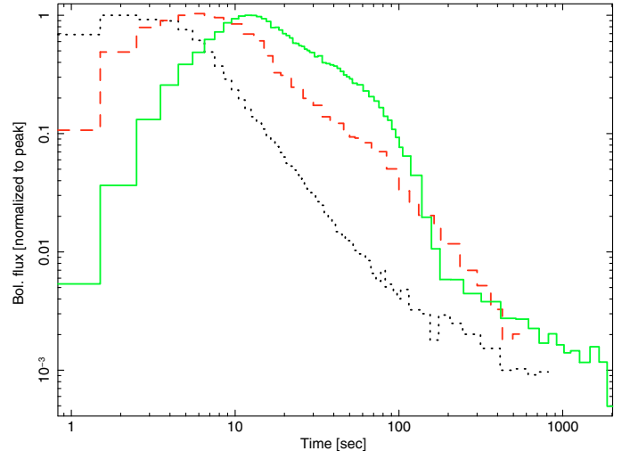
Fig. 14. The average time profiles of the bolometric flux for GS 1826-24 (solid green curve) and 4U 1728-34 (dotted black) and the profile for the triple burst from EXO 0748-676 (dashes red; the profile is cut at the time the 2nd burst occurs). Fluxes are renormalized with the respective peak values.
