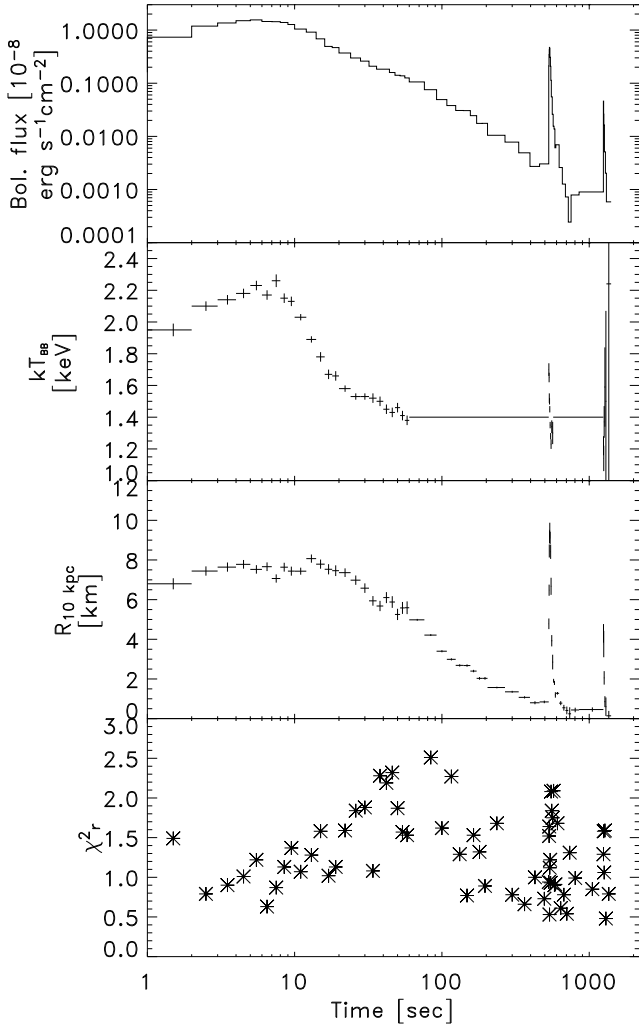
Fig. 9. Time-resolved spectroscopy of the triple burst from EXO 0748-676. A pre-burst spectrum was subtracted before fitting the spectra with an absorbed black body model with N_{\text{H}} = 8 \times 10^{21} \text{ cm}^{-2} . For data between 60 to 1200 s, we fixed kT for the tail emission to 1.4 keV, equal to the average value if kT is left free for the relevant time intervals.
