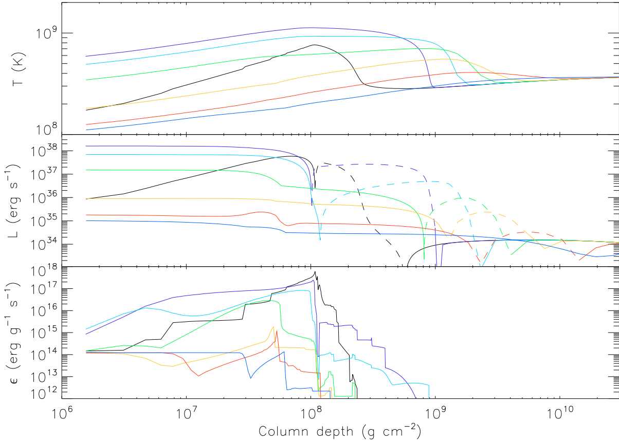
Fig. 11. Profiles of temperature ( top panel ), net outward luminosity ( middle ; dashed parts indicate inward luminosity) and specific nuclear energy generation rate ( bottom ) calculated as a function of depth for a flash model specifically for GS 1826-24 (model “A3” of Heger et al. 2007). Seven profiles are shown. The black curve is for t = 0 (burst onset), the other curves are for the times indicated with vertical lines in Fig. 10 with the same color. The top panel shows the inward heating (compare with the location of the heat source in the bottom panel , down to only 9 \times 10^8 \text{ g cm}^{-2} ) that is thought to be responsible for the long tails on the X-ray bursts of GS 1826-24. See also Fig. 12. The color version of this figure is only available online.
