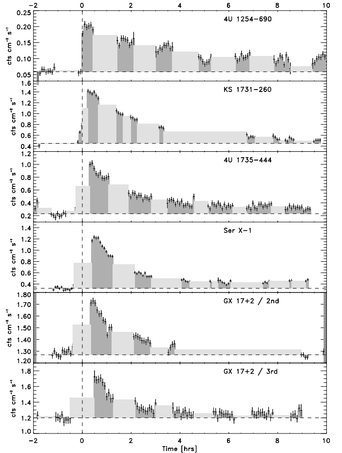
Fig. 7. 2–28 keV light curves of 2 superbursts from GX 17+2 compared with those of the other superbursters detected with the WFCs. The e-folding decay times are from top to bottom 6.0 h (4U 1254–69; In 't Zand et al. 2003a), 2.7 h (KS 1731–260; Kuulkers et al. 2002a), 1.4 h (4U 1735–444; Cornelisse et al. 2000), 1.2 h (Ser X–1; Cornelisse et al. 2002), 1.9 h (GX 17+2, 2nd superburst) and 1.0 h (GX 17+2, 3rd superburst). The horizontal dashed lines indicate the pre-burst flux level, the vertical dashed lines the best estimate for the burst onsets, and the light grey regions represent flux estimates during data gaps being averages of the last data point before the data gap and the first after.
