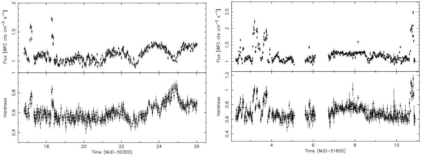
Fig. 1. Flux and 2–6/6–25 keV spectral hardness ratios of GX 17+2 during two nine-day long observations in August 1996 ( left ) and September 1999 ( right ). WFC unit 2 was employed in both observations. The time resolution is 15 min.
