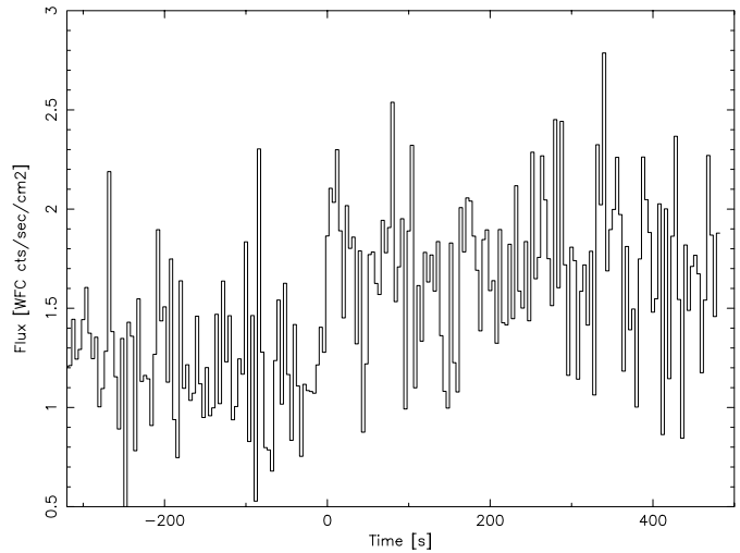
Fig. 5. Rising part of flare 6 at 4-s resolution.
