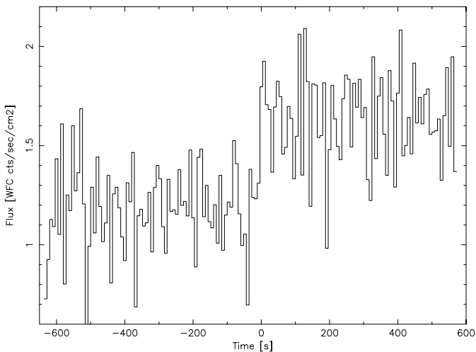
Fig. 4. Rising part of flare 4 at 8-s resolution.
