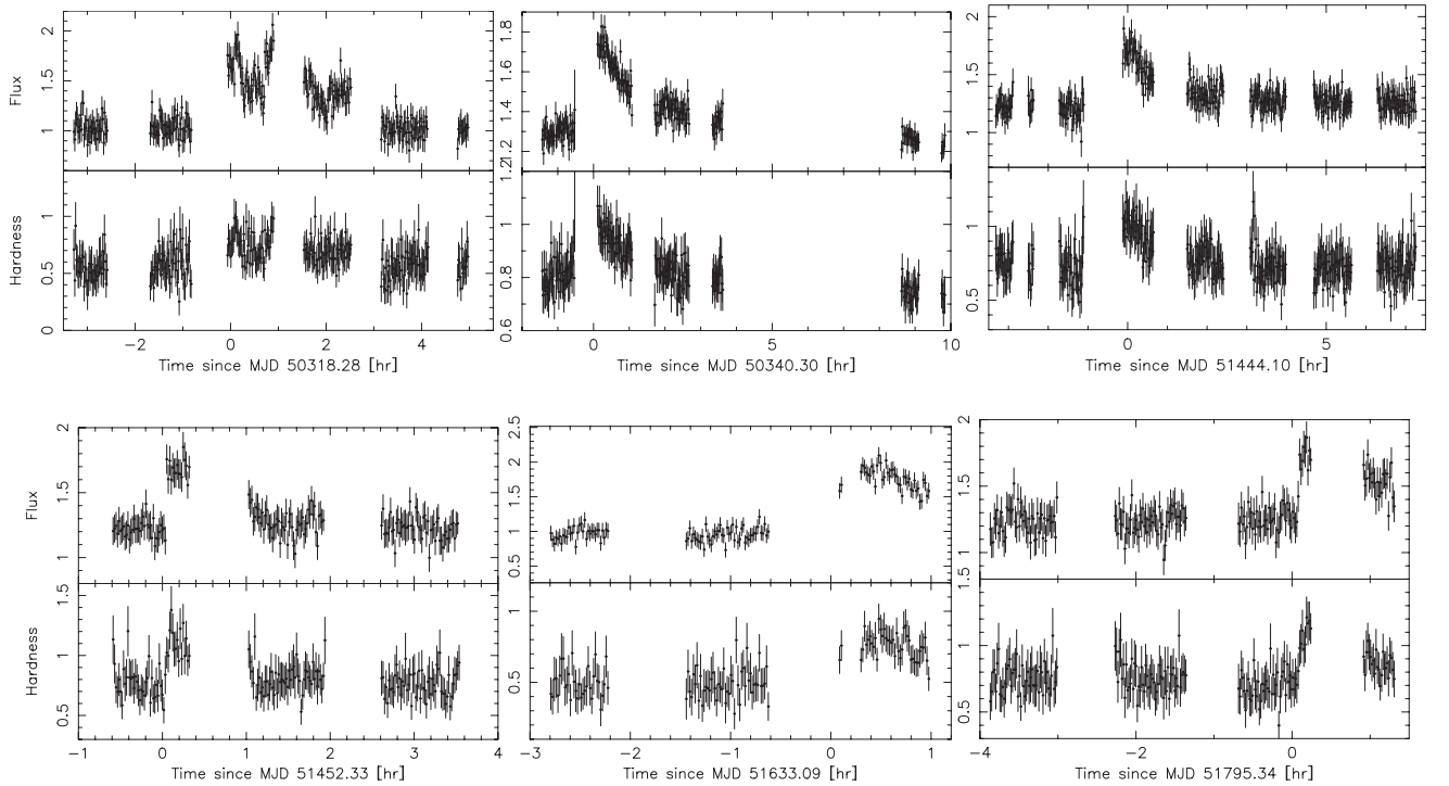
Fig. 2. 2–28 keV flux and 2–6/6–28 keV hardness histories of all 6 isolated flares from GX 17+2 with 64 s time resolution. All data of each flare are plotted (which is somewhat limited in the last two flares).
